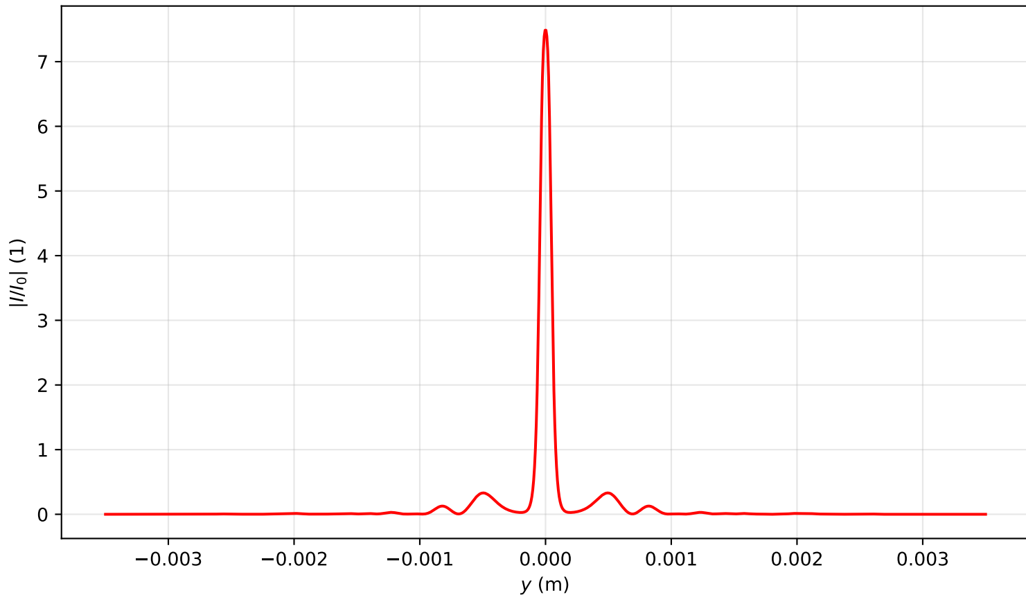
Intensity profile I(x=0, y, z=0.478)/I_0 , \text{Pin}=9.0\text{Pcr} , artificial time
